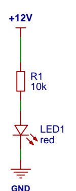
POWER SUPPLY / FILTERING / POWER LED
