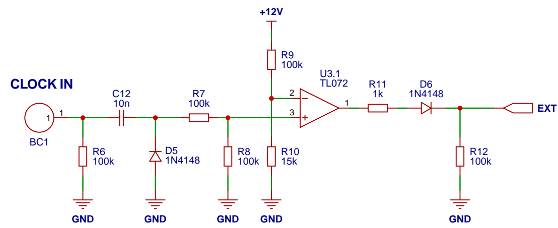
EXTERNAL CLOCK
